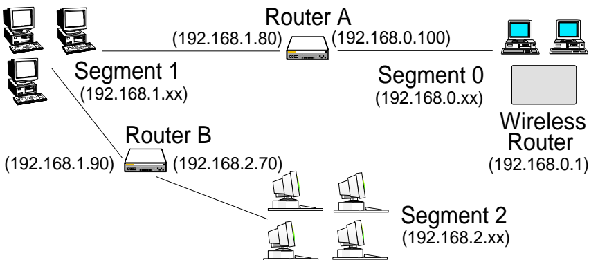
Figure 46: Routing Example
